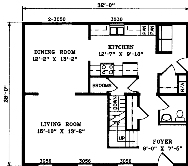
1ST STORY FLOOR PLAN---BASEMENT MODEL
