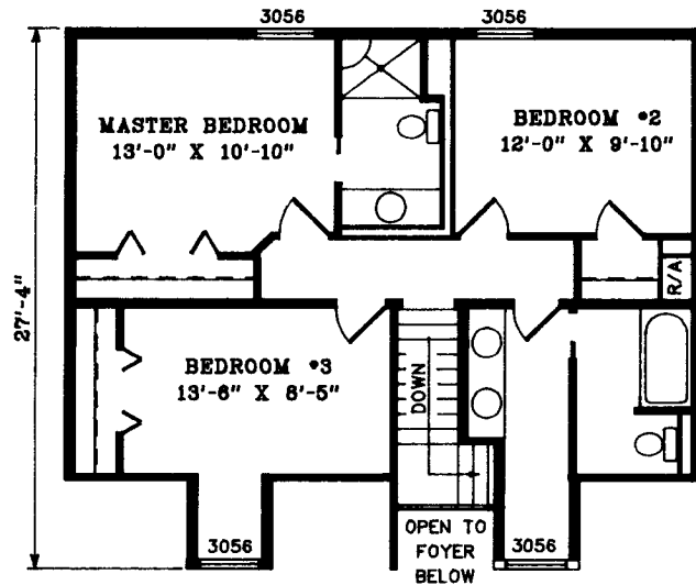
2ND STORY FLOOR PLAN
