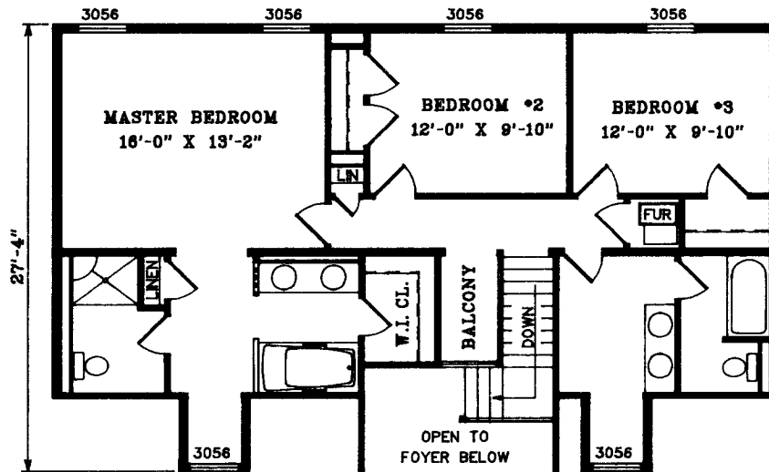
2ND STORY FLOOR PLAN
