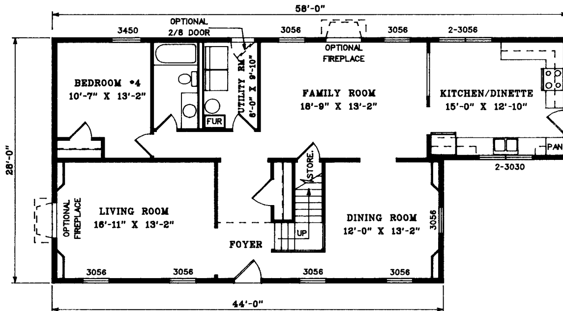
1ST STORY FLOOR PLAN---CRAWLSPACE MODEL
