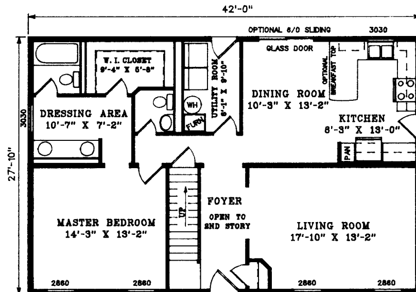
1ST STORY FLOOR PLAN
