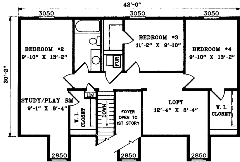
2ND STORY FLOOR PLAN
