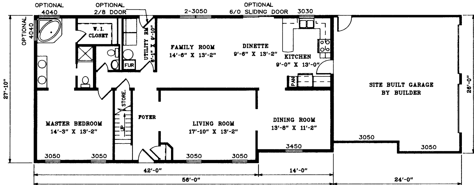
1ST STORY FLOOR PLAN---CRAWLSPACE MODEL
