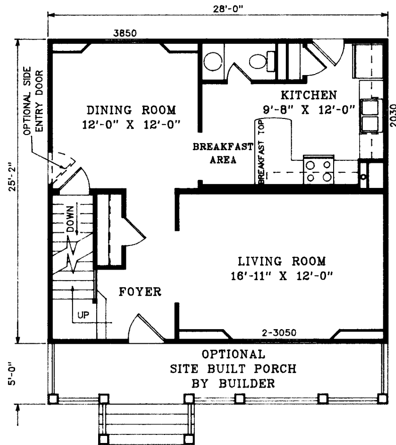
1ST STORY FLOOR PLAN
