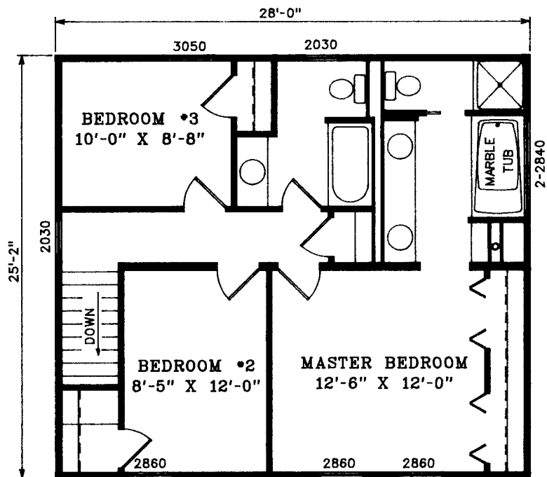
2ND STORY FLOOR PLAN
