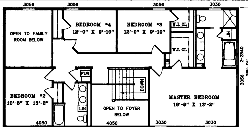
2ND STORY FLOOR PLAN
