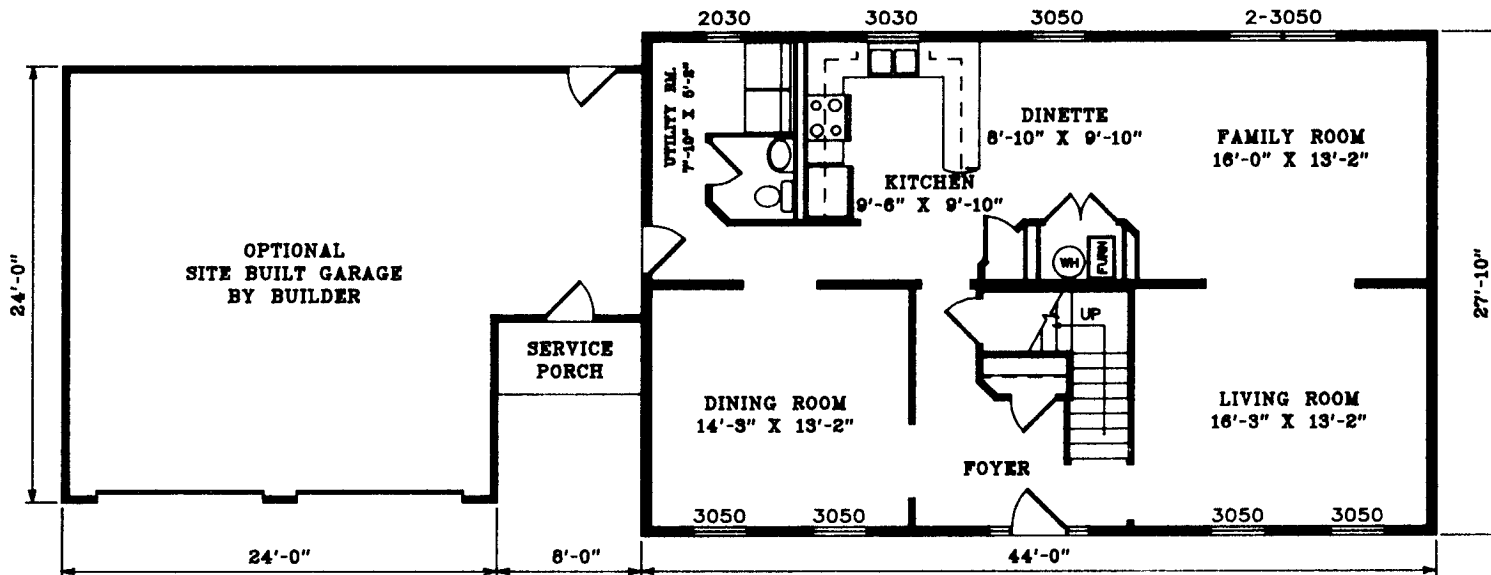
1st FLOOR ON CRAWLSPACE FOUNDATION
