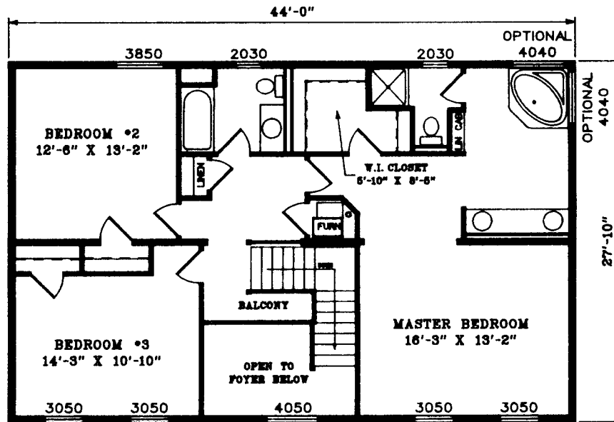
2nd FLOOR
