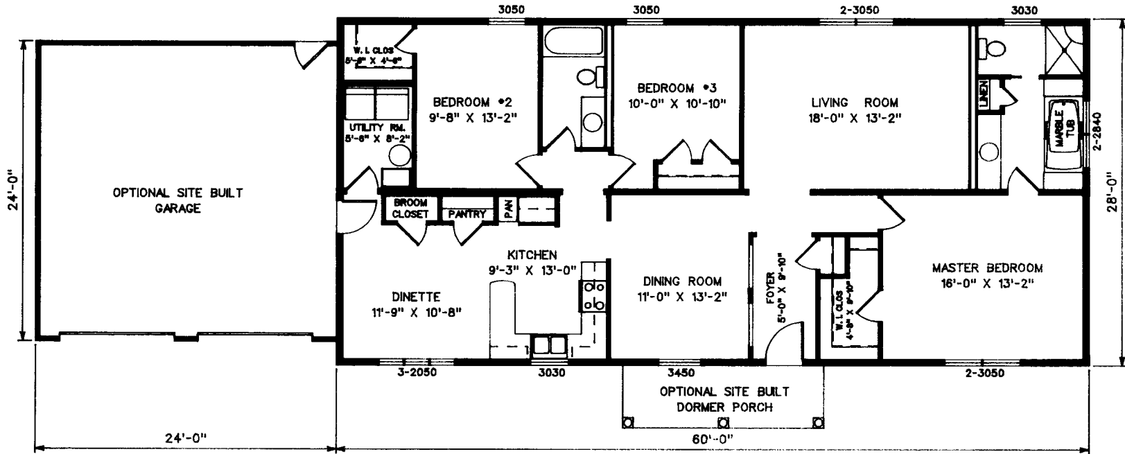
CRAWLSPACE MODEL
