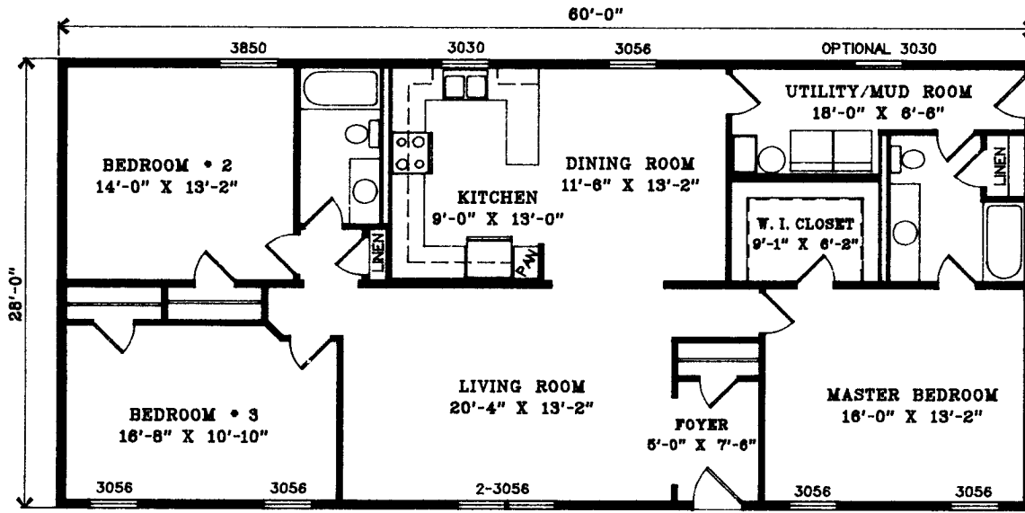
CRAWLSPACE MODEL (SIDE GARAGE ADAPTABLE)
