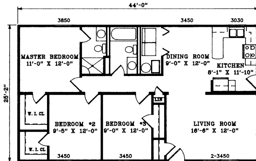
CRAWLSPACE MODEL (SIDE GARAGE ADAPTABLE)
