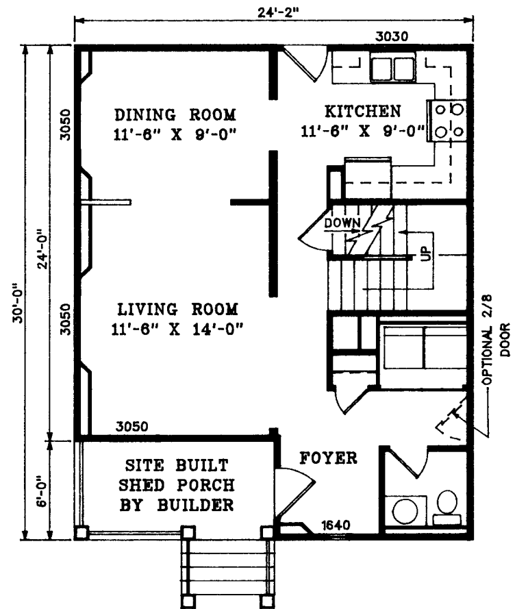
1ST STORY FLOOR PLAN
