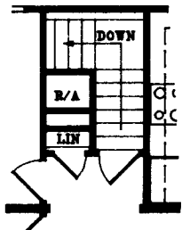
BASEMENT MODEL
