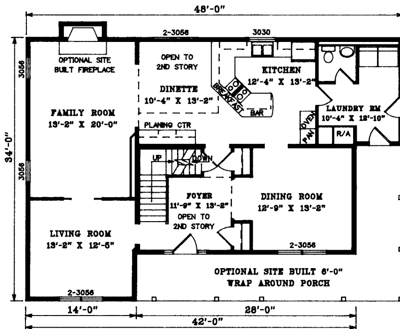
1ST STORY FLOOR PLAN---BASEMENT MODEL
